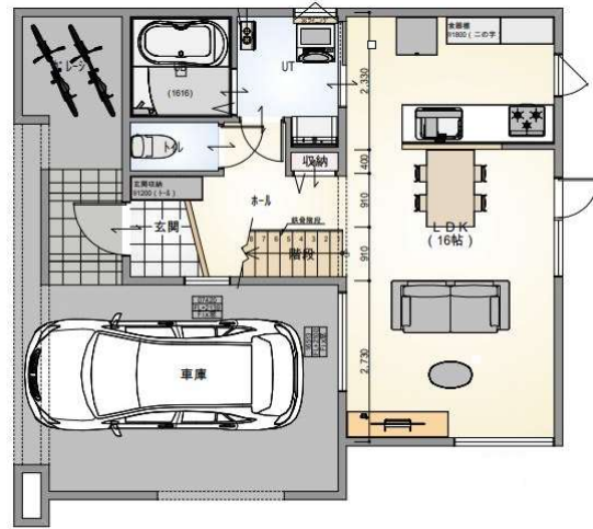
1F PLAN
