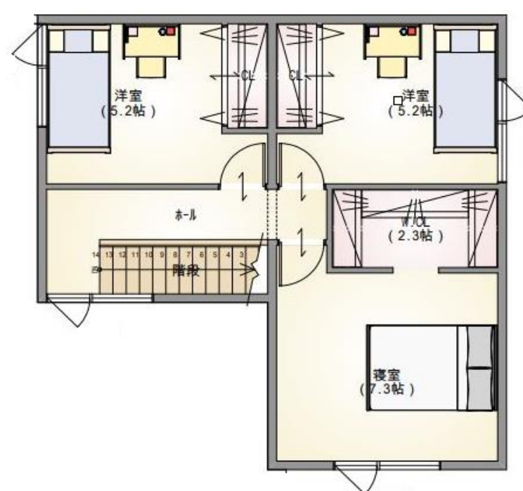
2F PLAN
