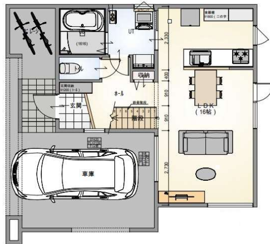
1F PLAN
