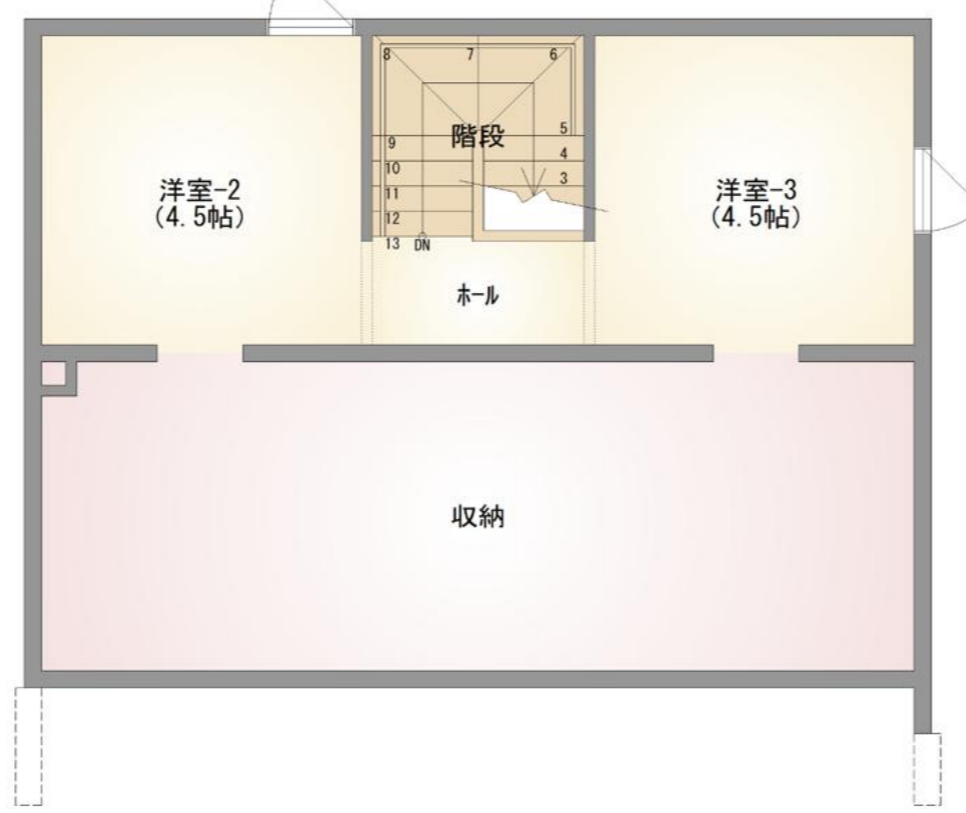
2F PLAN
